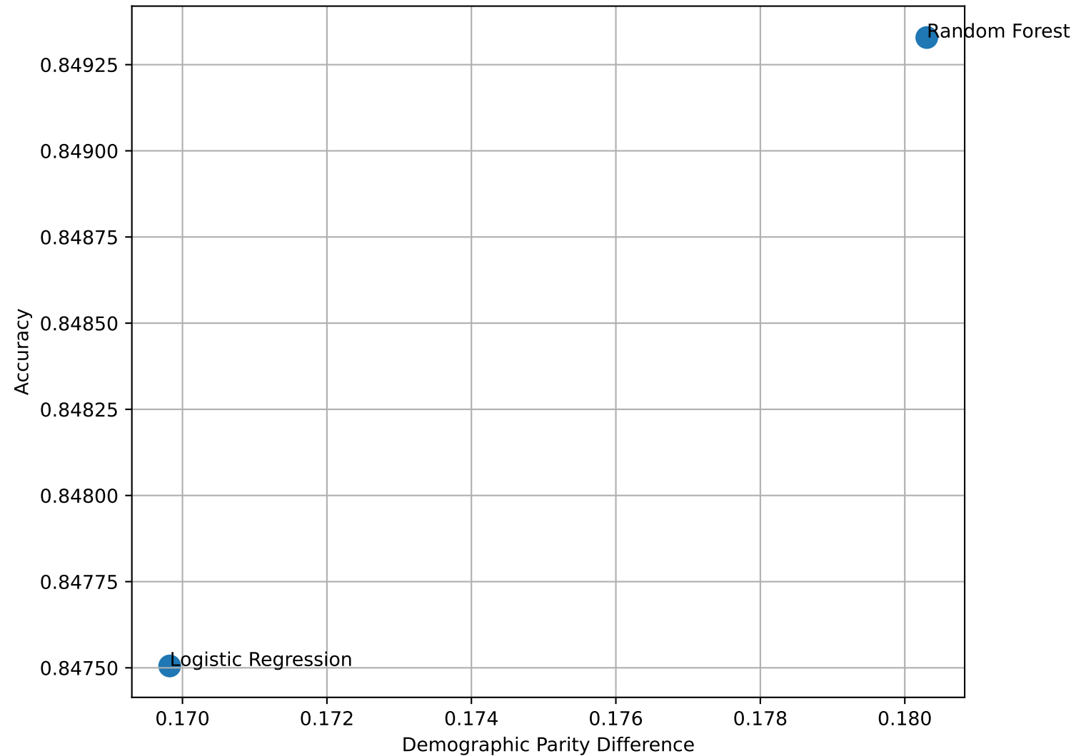
RQ1: Fairness vs Accuracy Trade-off
